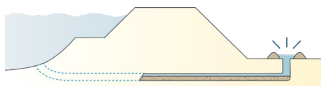
Piping
